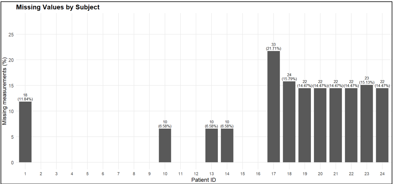
Figure 2. Percentage of missing craniofacial measurements by subject. Labels indicate the number and percentage of missing measurements for each subject.
