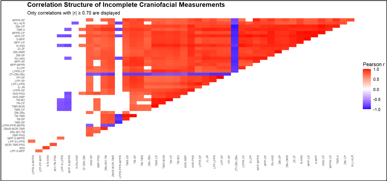
Figure 4. Correlation structure among craniofacial measurements containing missing values. Only Pearson |r| \geq 0.70 correlations with are displayed.
