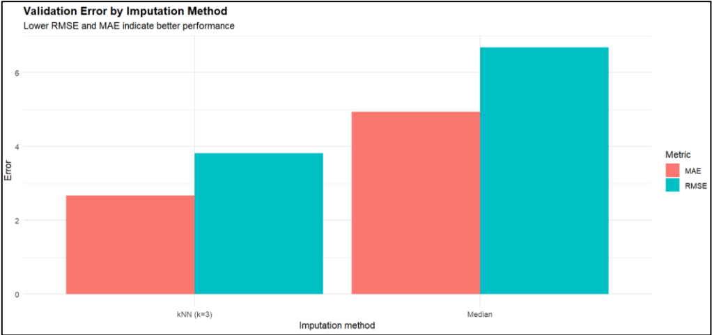
Figure 5. Validation performance of median and kNN imputation based on artificially masked observed values. Lower RMSE and MAE indicate better predictive performance.
