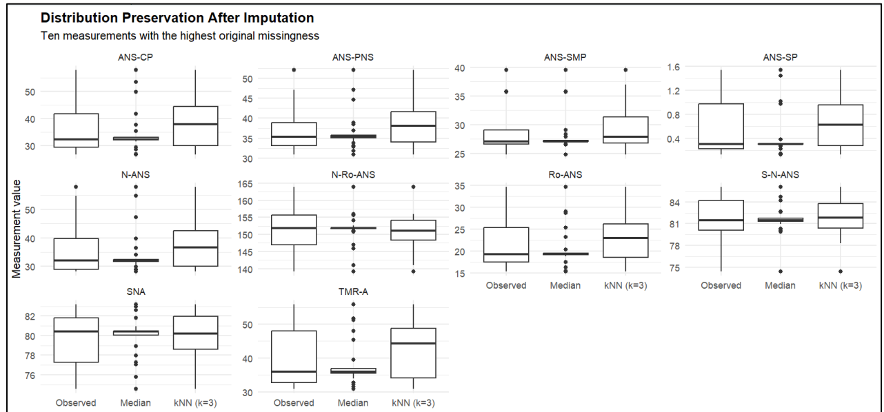
Figure 6. Distribution of observed and imputed values for the ten craniofacial measurements with the highest original missingness. Median imputation generally reduced variability, whereas kNN () preserved the observed distributions more closely.
