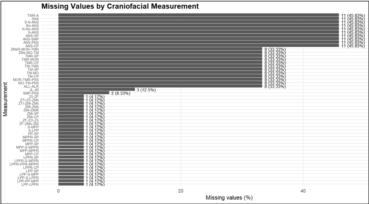
Figure 1. Percentage of missing values by craniofacial measurement. Only measurements with at least one missing observation are shown; labels indicate the number and percentage of missing observations.
