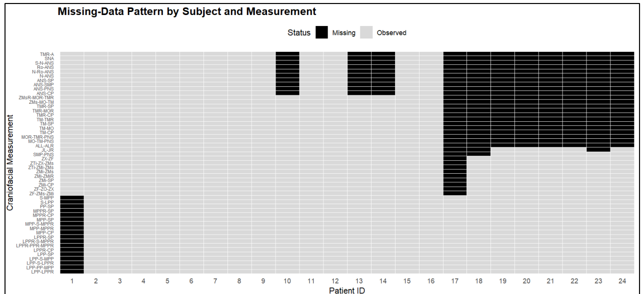
Figure 3. Missing-data pattern by subject and craniofacial measurement. Black cells indicate missing observations and grey cells indicate observed observations. Only measurements with at least one missing value are displayed.
